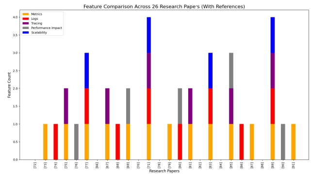
FIGURE 5. Frameworks' feature comparison.
